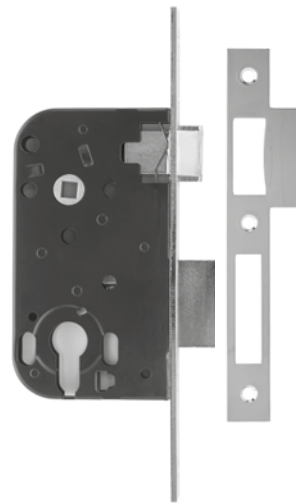
CYLINDRE | CYLINDER
