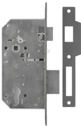
CYLINDRE | CYLINDER
